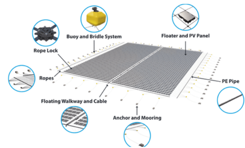
Modular floating PV system for nearshore applications
