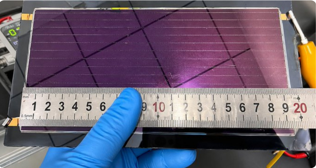
27.39%-efficient inverted perovskite solar cell based on new molecular design
